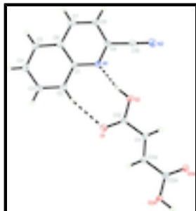
Fig. 1. The molecular structure of the title compound showing 50% probability displacement ellipsoids for non-H atoms and the atom-numbering scheme. Atoms with suffix A were generated by the symmetry code -x, -y + 1, -z + 1 . Hydrogen atoms are shown as spheres of arbitrary radius.
